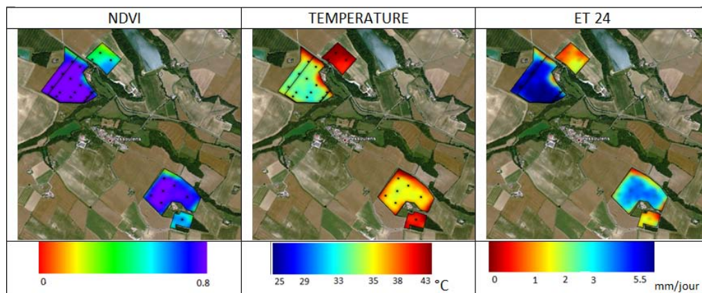
Fig. 4. Example of pictures sent to the farmer 3 days after taken by the satellite and showing on the left NDVI, center the temperature and right the ET computed with SEBAL
