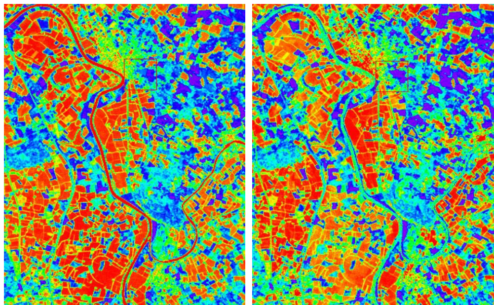
Fig.3. Map of NDVI (left) and NDWI (right) computed over Middle Garonne from a Landsat picture taken on 2011 April 9 th .
